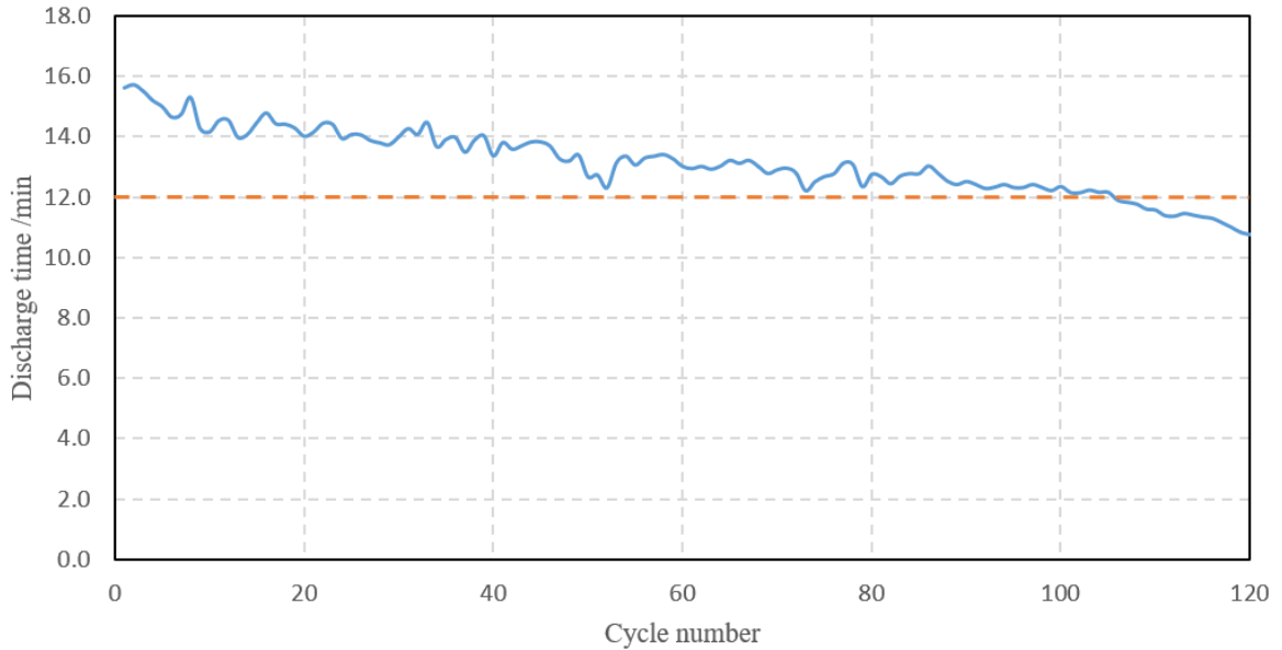
Graph 1 HRL series 15min constant power discharge curve at 25 DegC
