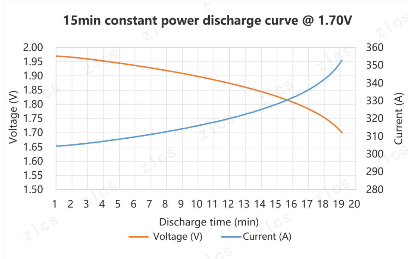
Graph 2 HRL series 15min Discharge Voltage and Current curve at 25 DegC
