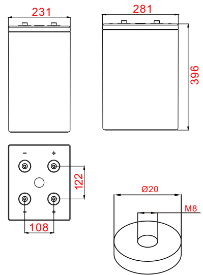
Terminal Dimensions
