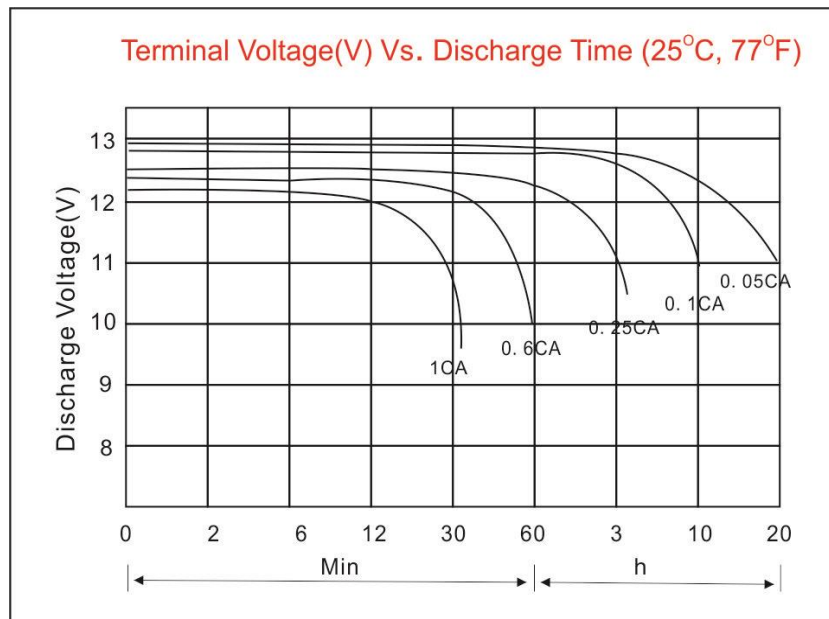
Fig. 2-2 Discharge Curves at different current at 25°C
