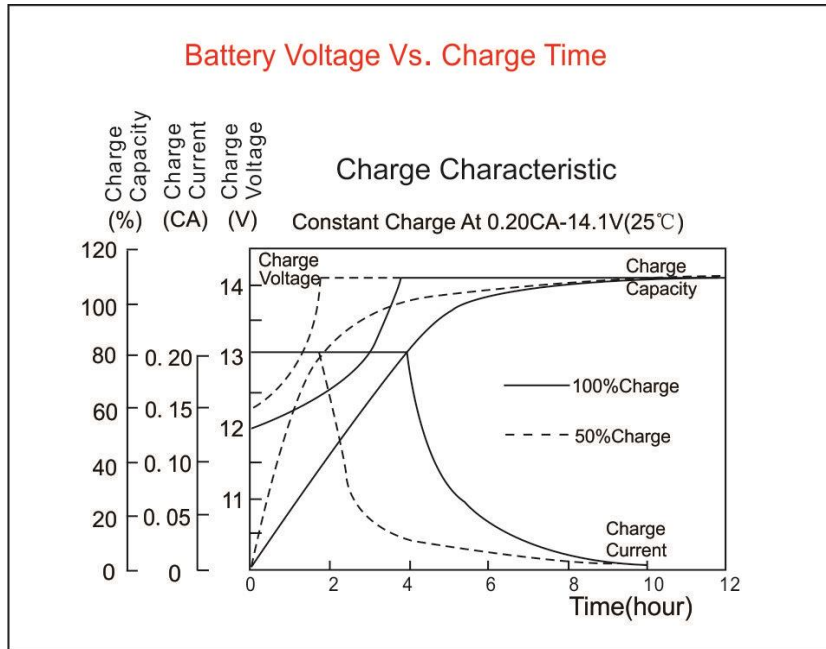
Fig. 2-1 The battery voltage vs charge time curves at 25°C
